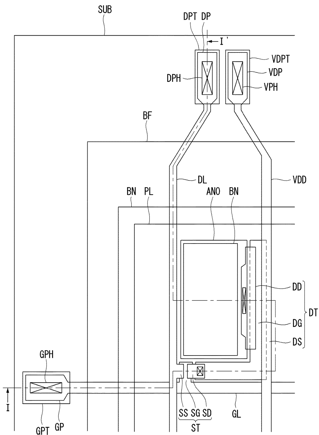
Related Art
